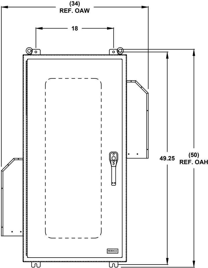
FRONT VIEW
