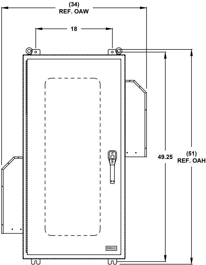
FRONT VIEW
