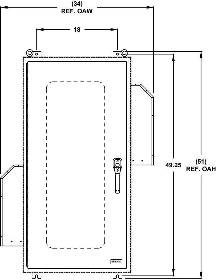
FRONT VIEW
