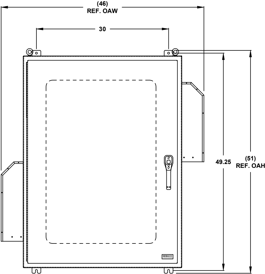
FRONT VIEW
