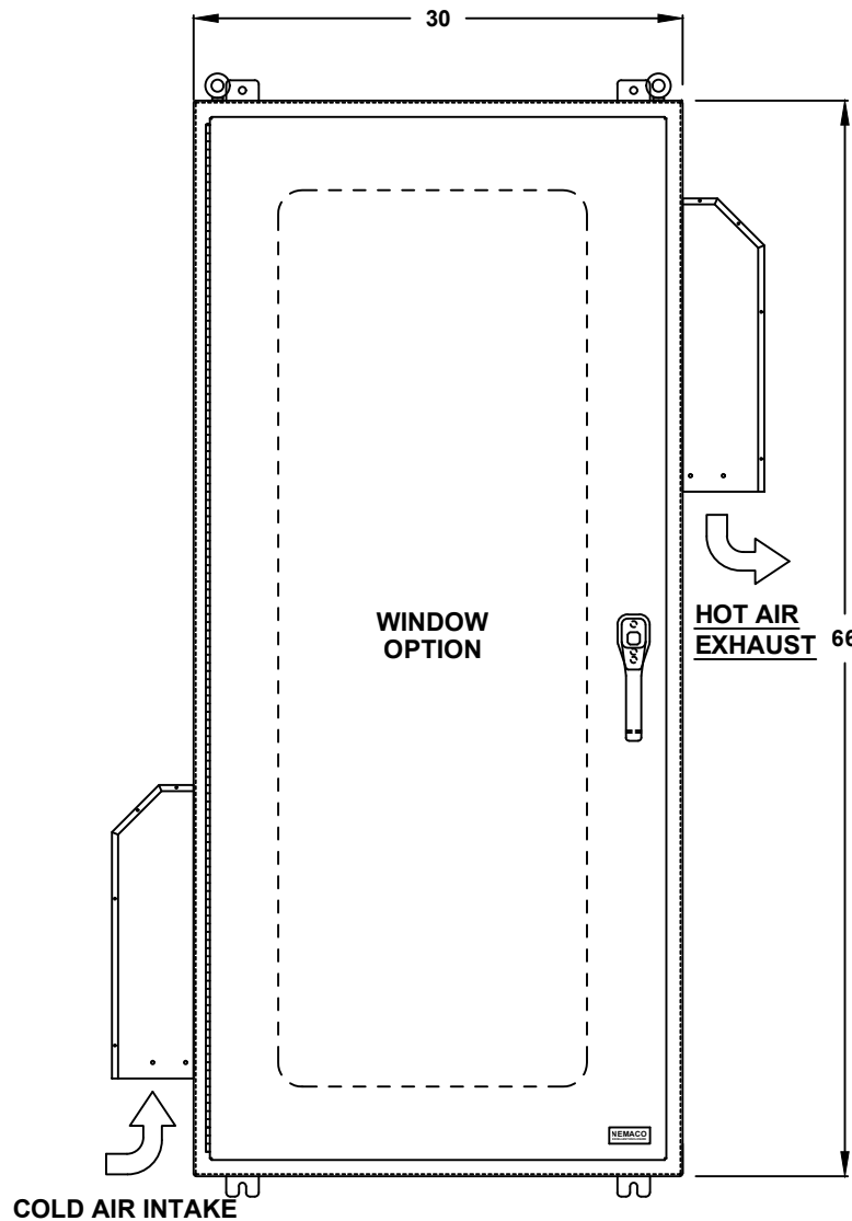
FRONT VIEW
