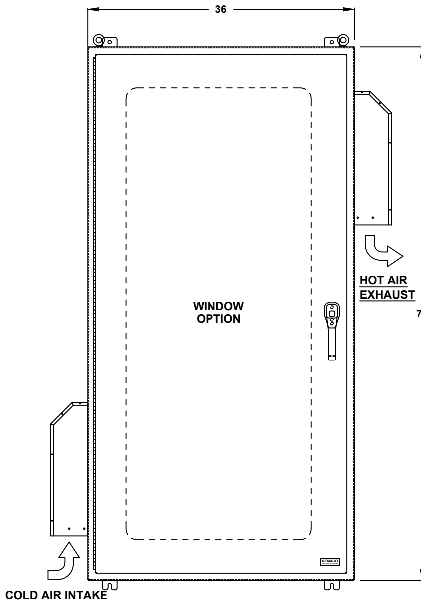
FRONT VIEW
