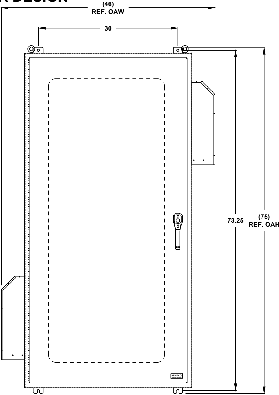
FRONT VIEW
