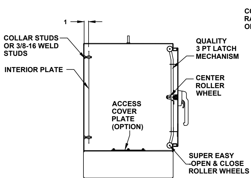
CROSS SECTION VIEW A-A
