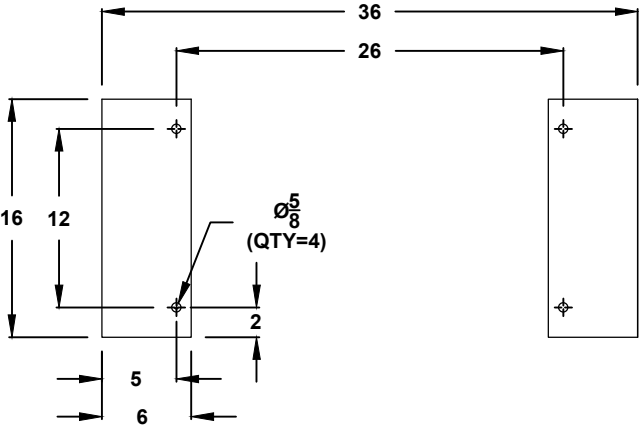
CROSS SECTION VIEW C-C MOUNTING HOLES
