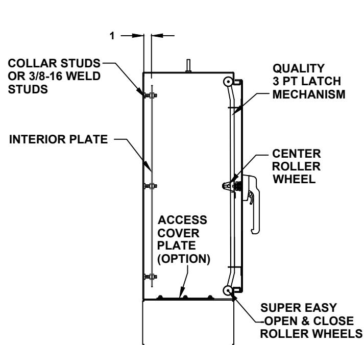
CROSS SECTION VIEW A-A
