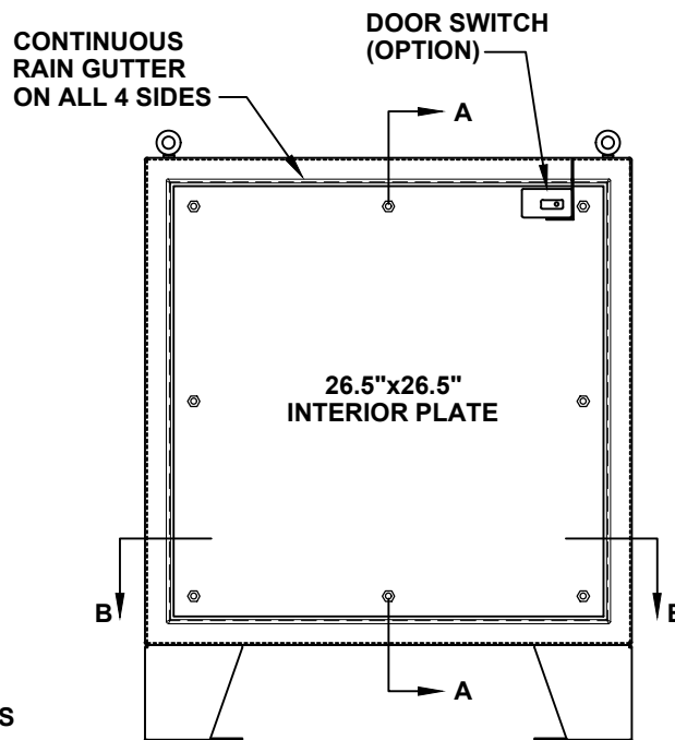
FRONT VIEW WITH DOOR REMOVED
