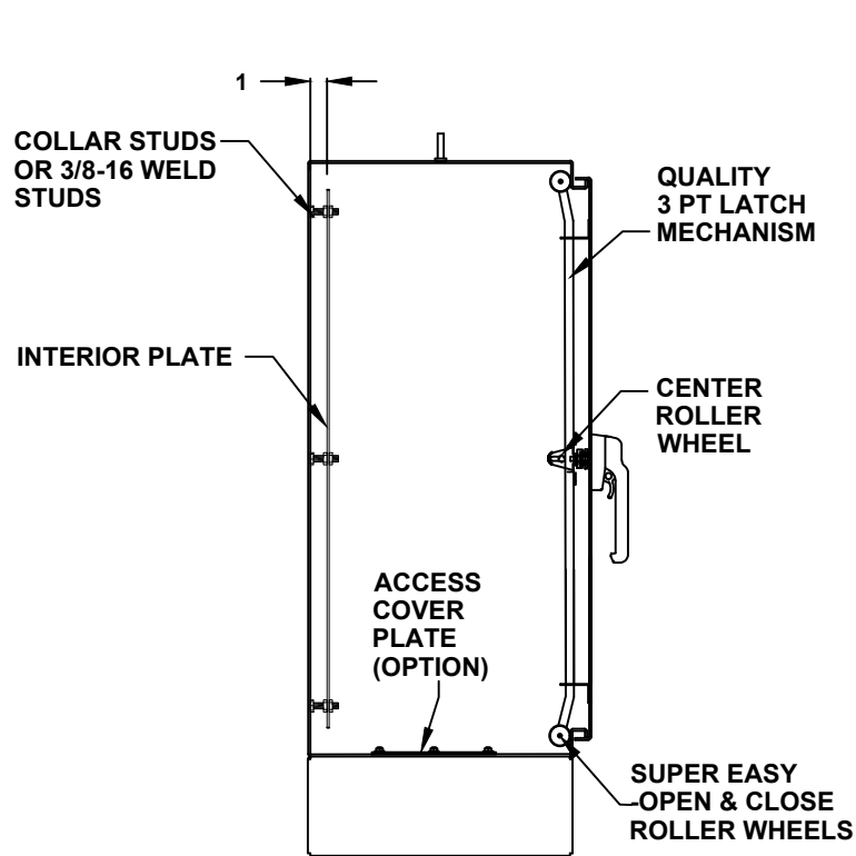
CROSS SECTION VIEW A-A
