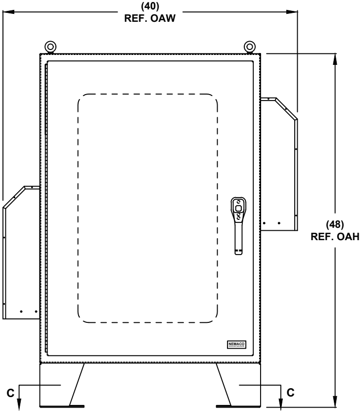
FRONT VIEW
