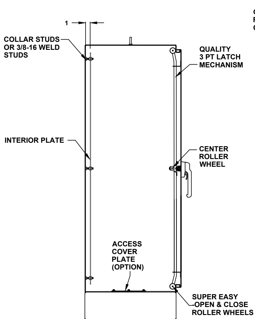
CROSS SECTION VIEW A-A
