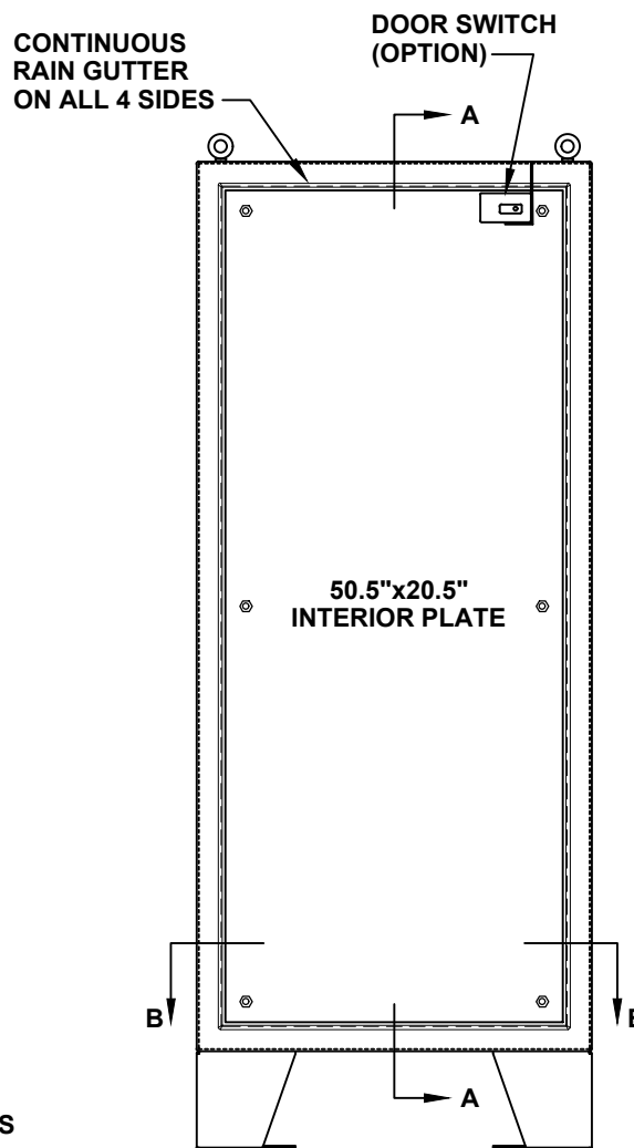
FRONT VIEW WITH DOOR REMOVED
