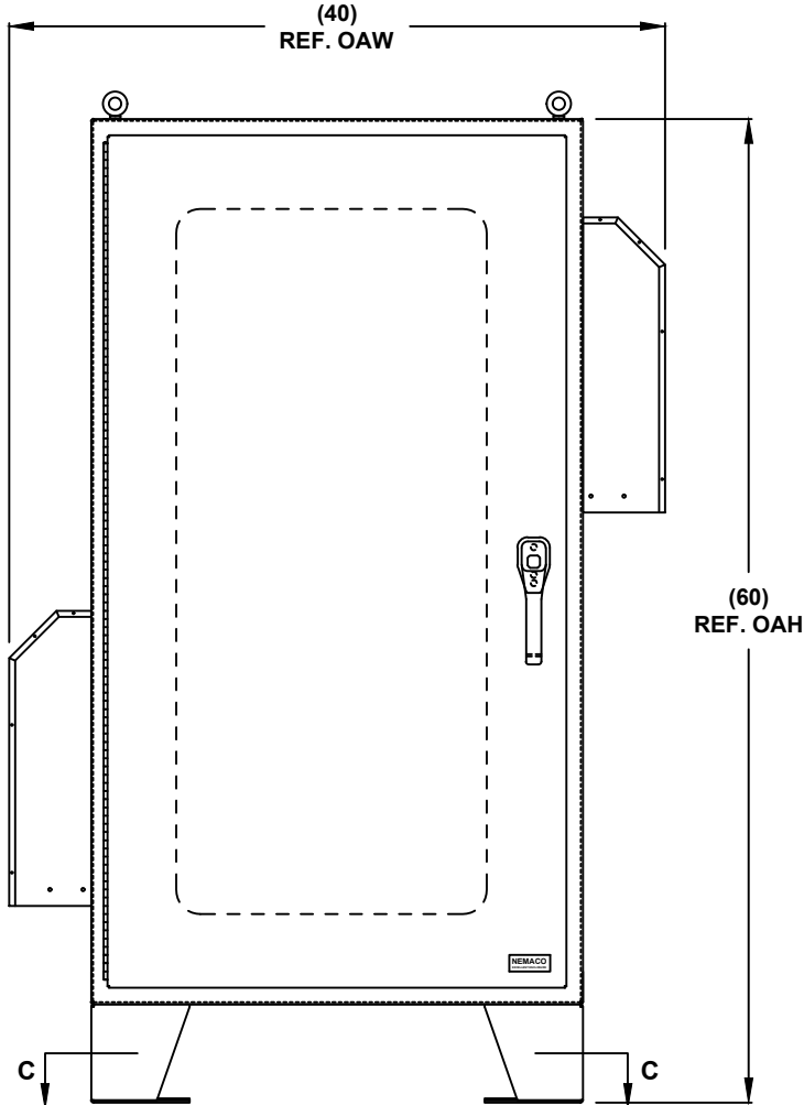
FRONT VIEW
