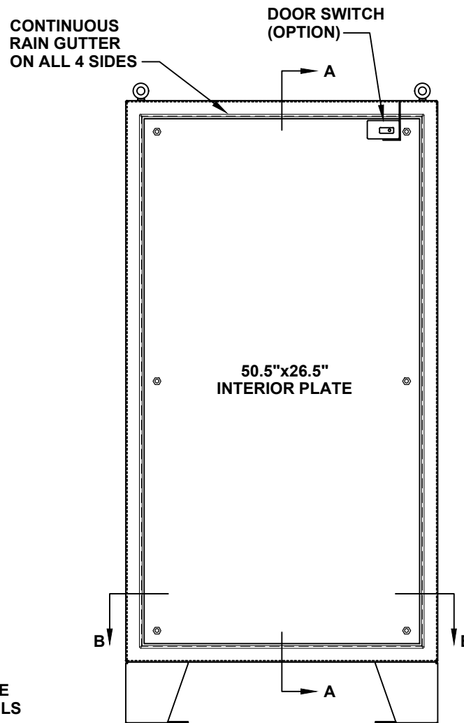
FRONT VIEW WITH DOOR REMOVED
