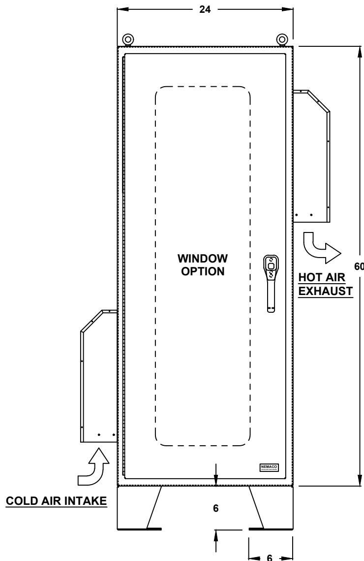
FRONT VIEW
