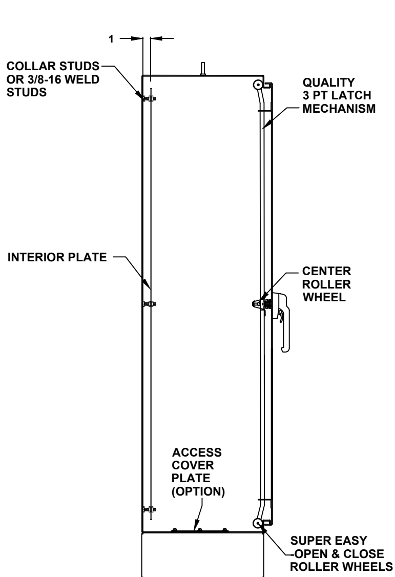
CROSS SECTION VIEW A-A
