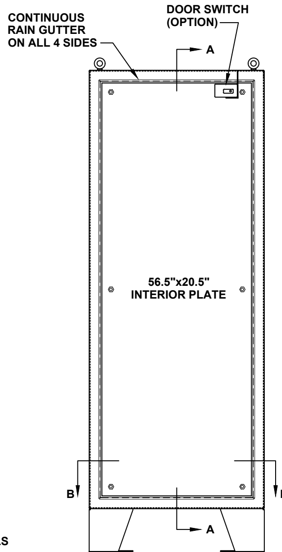
FRONT VIEW WITH DOOR REMOVED
