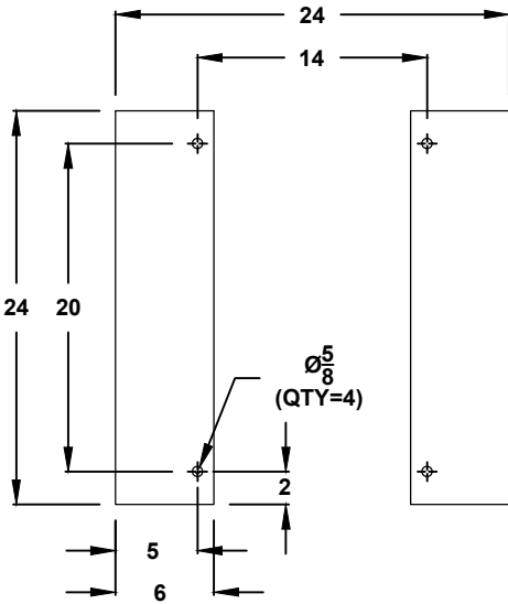
CROSS SECTION VIEW C-C MOUNTING HOLES
