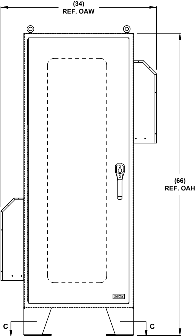
FRONT VIEW
