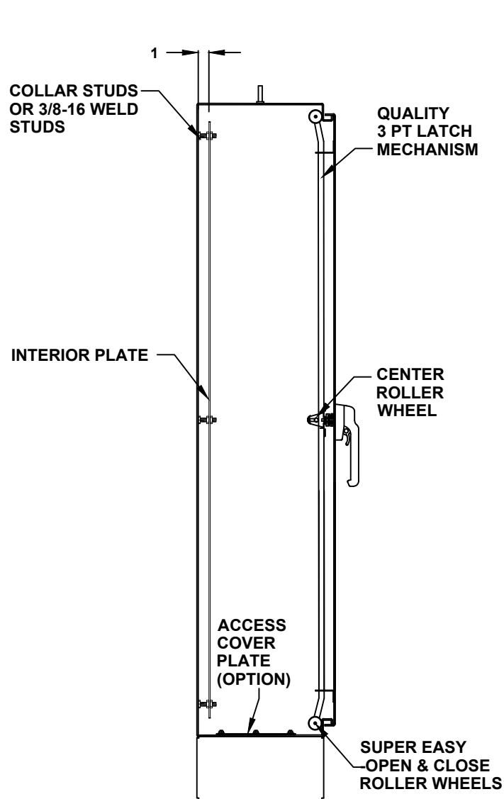
CROSS SECTION VIEW A-A
