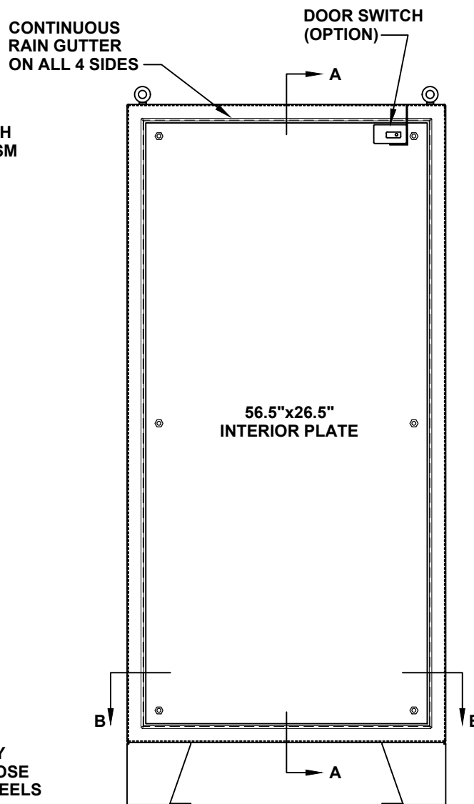
FRONT VIEW WITH DOOR REMOVED
