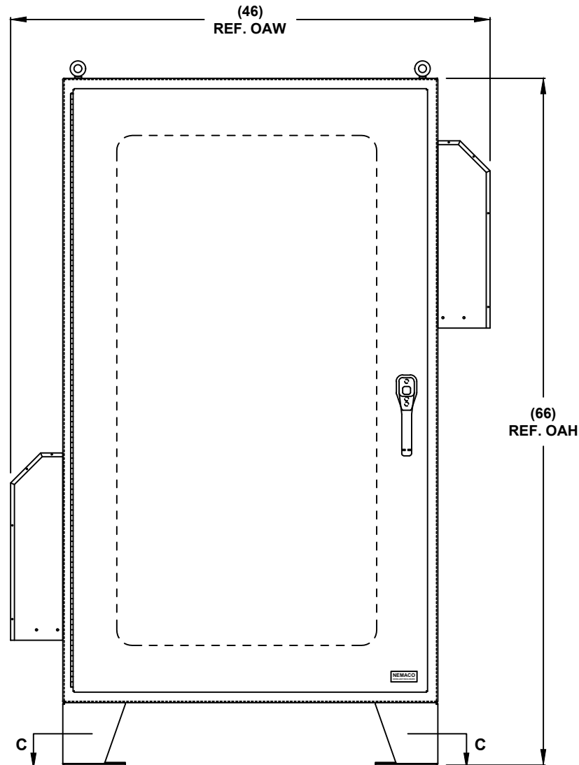
FRONT VIEW
