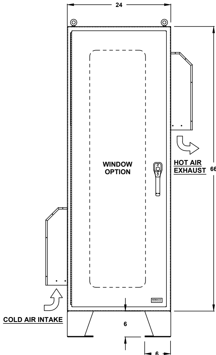
FRONT VIEW
