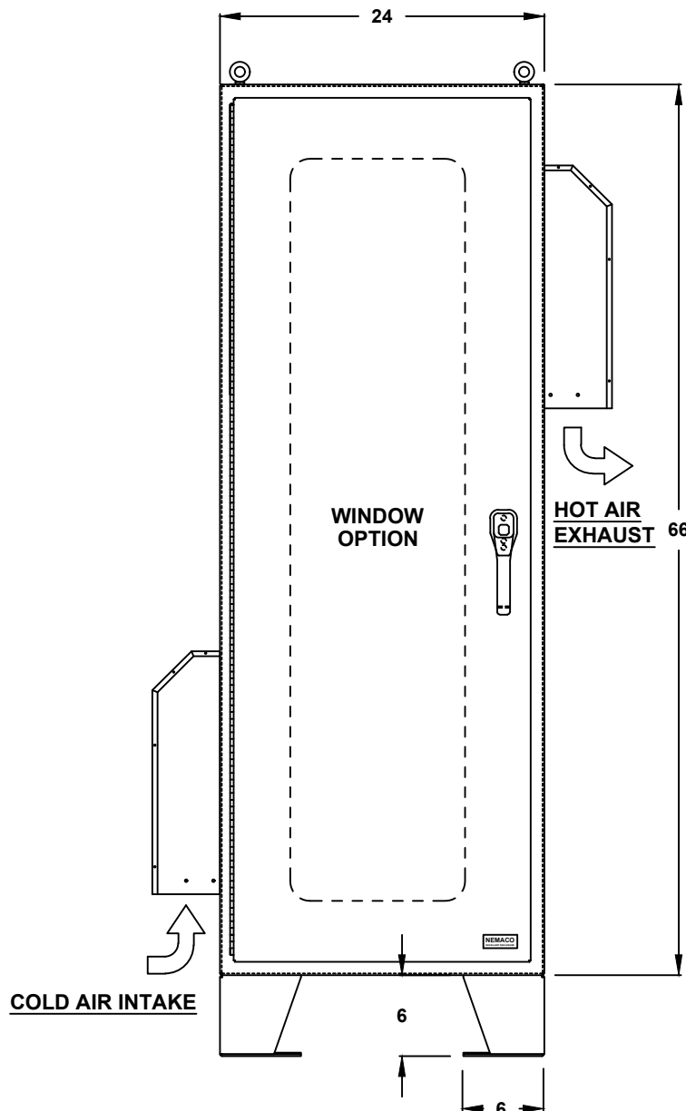
FRONT VIEW
