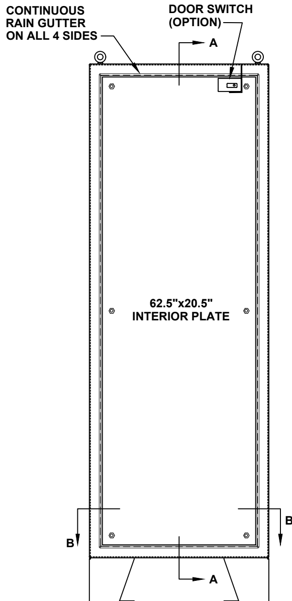
FRONT VIEW WITH DOOR REMOVED
