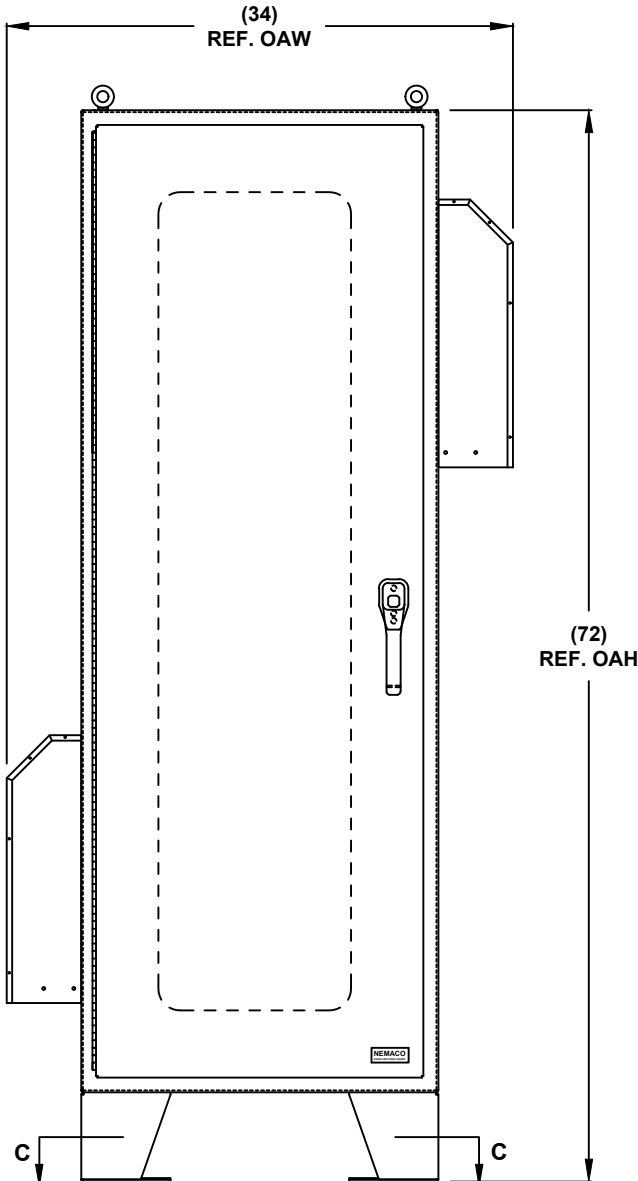
FRONT VIEW
