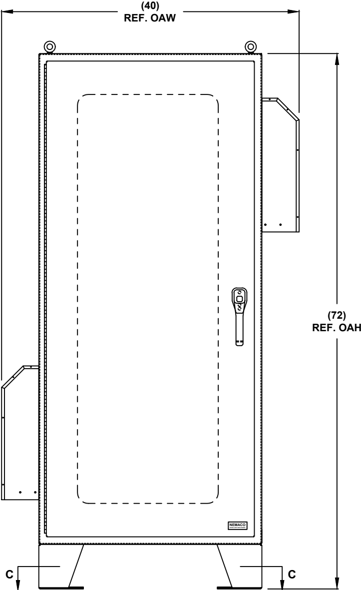
FRONT VIEW
