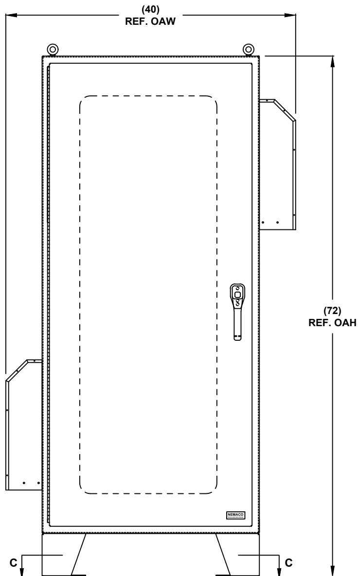
FRONT VIEW
