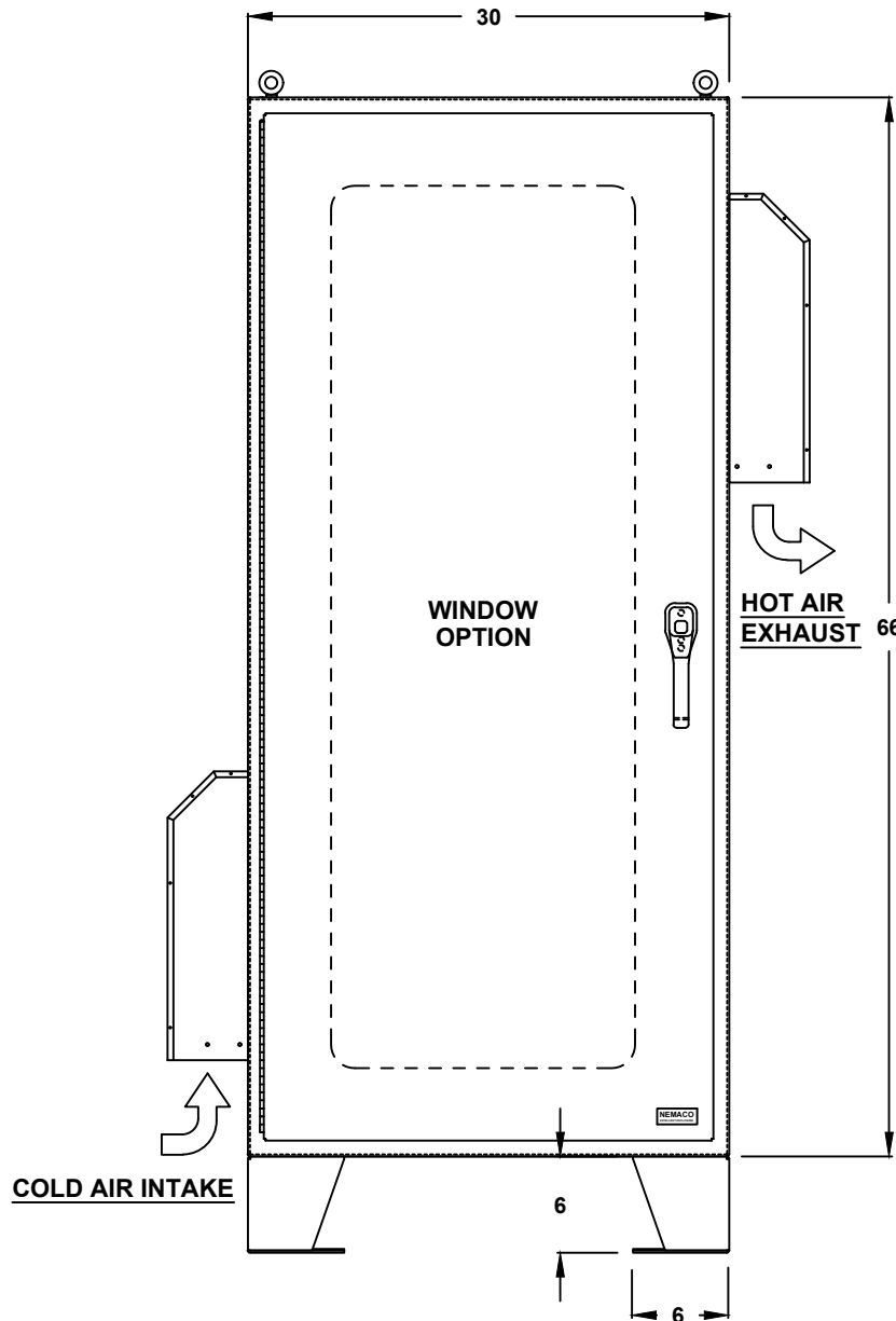
FRONT VIEW
