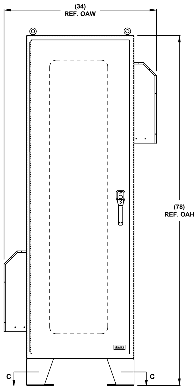
FRONT VIEW NEMACO™ ©2025
