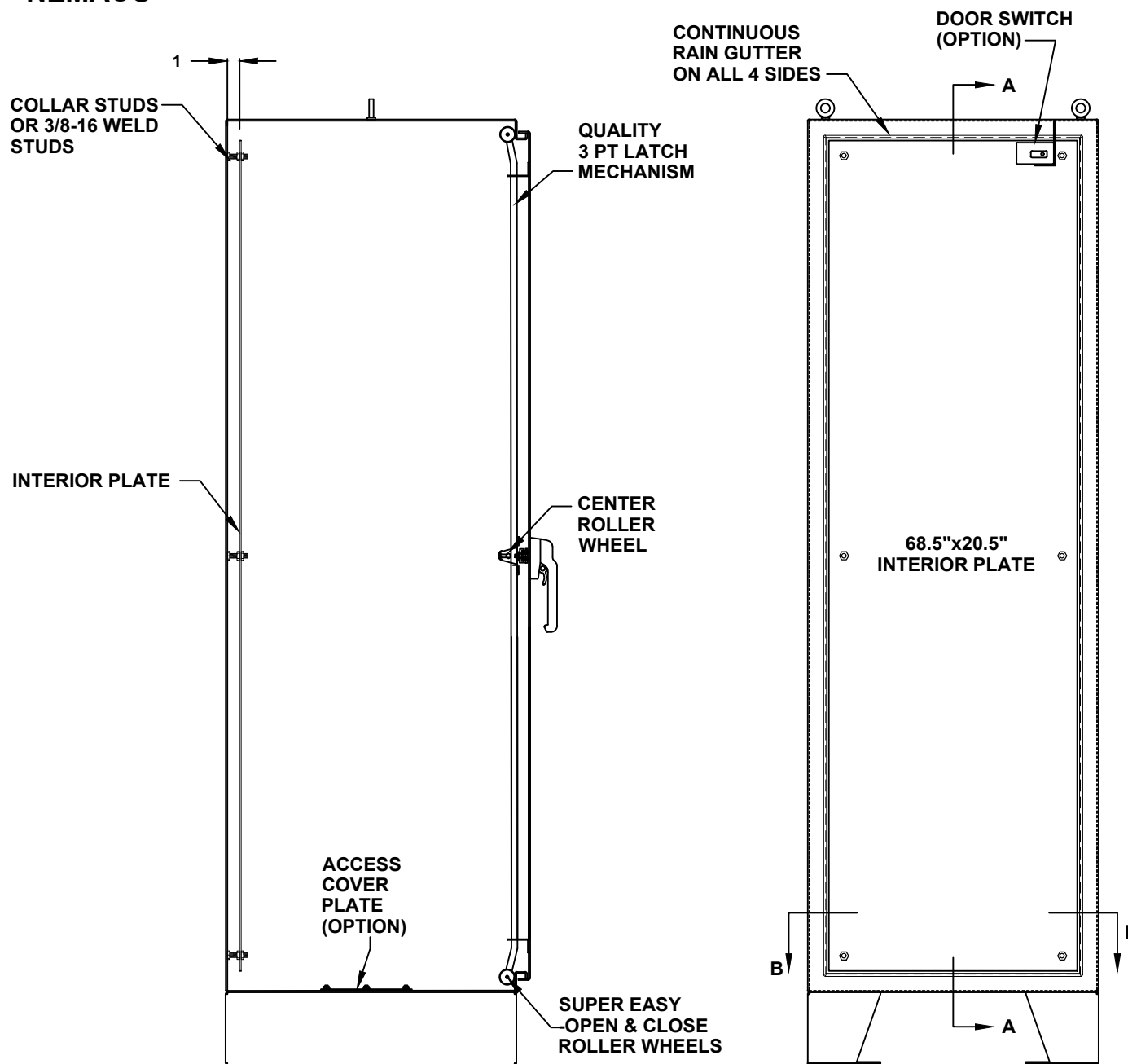
CROSS SECTION VIEW A-A
