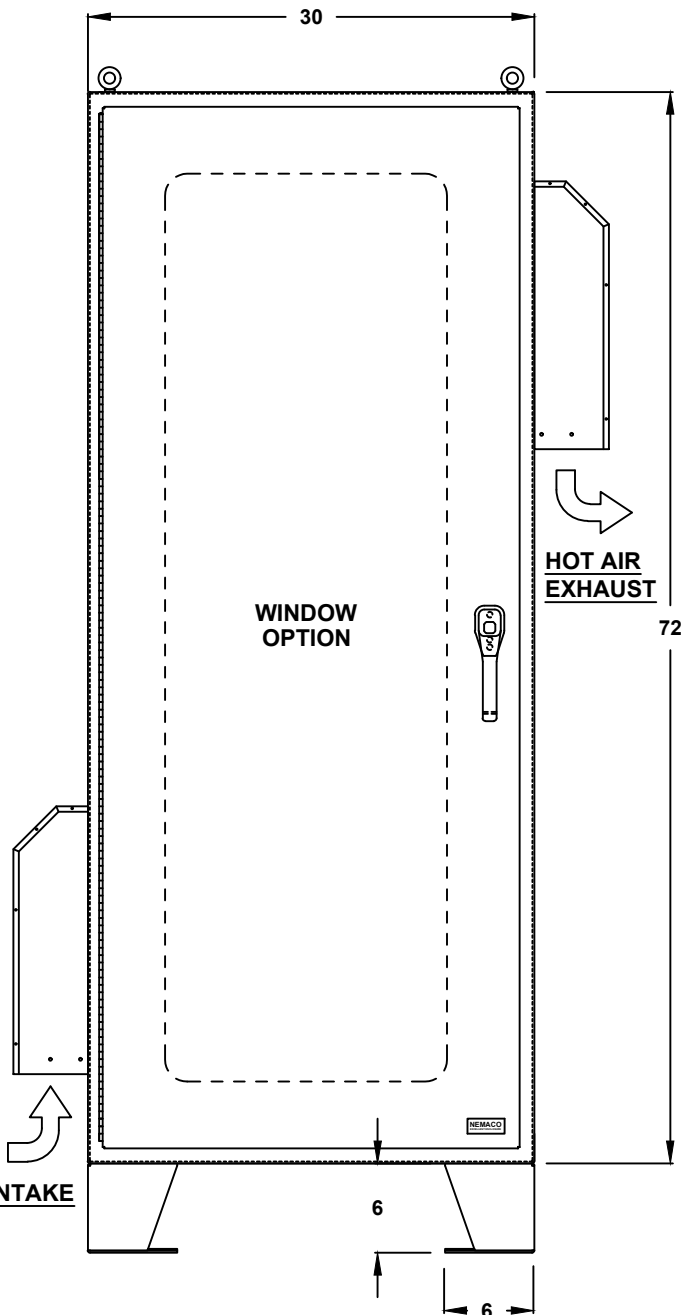
FRONT VIEW
