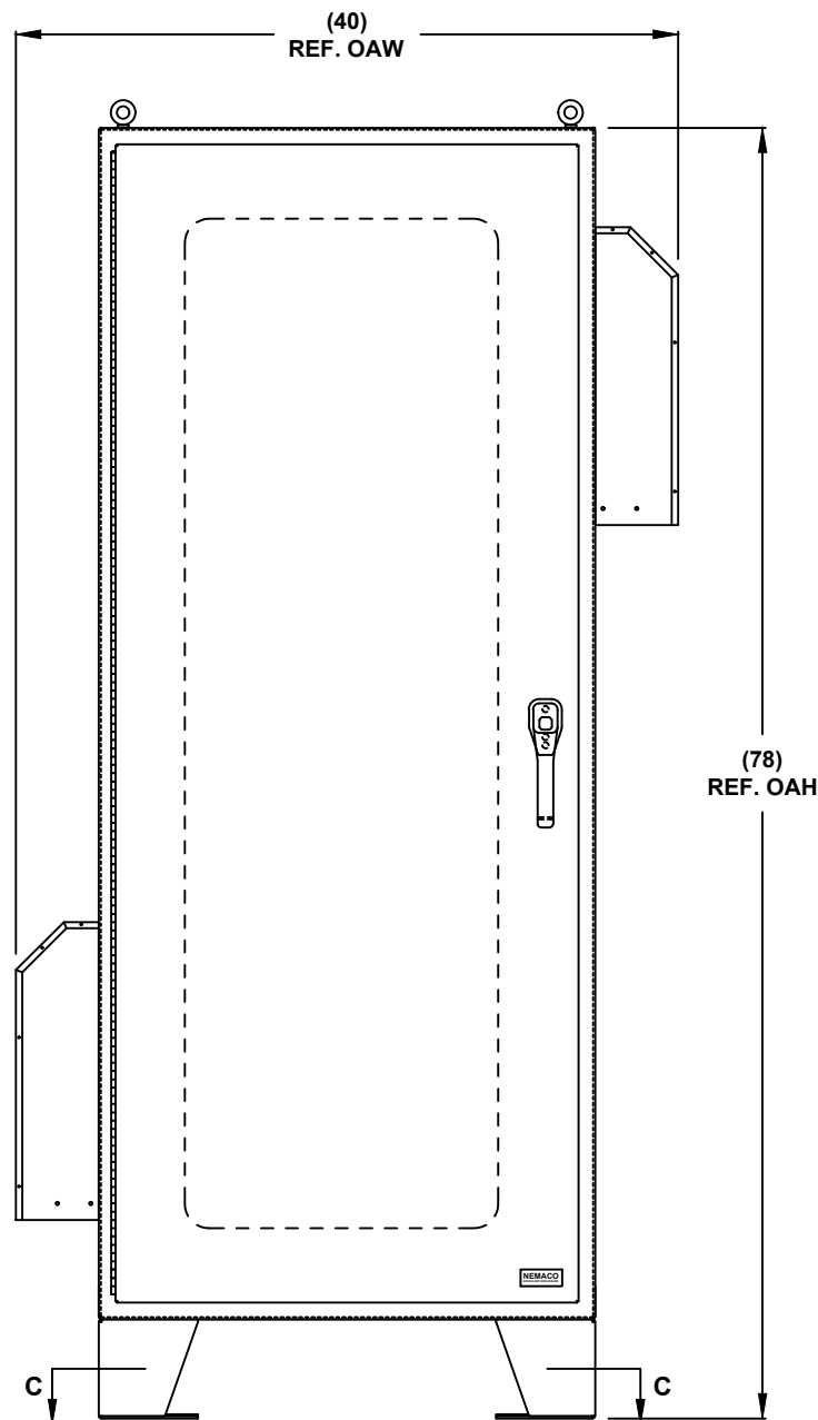
FRONT VIEW
