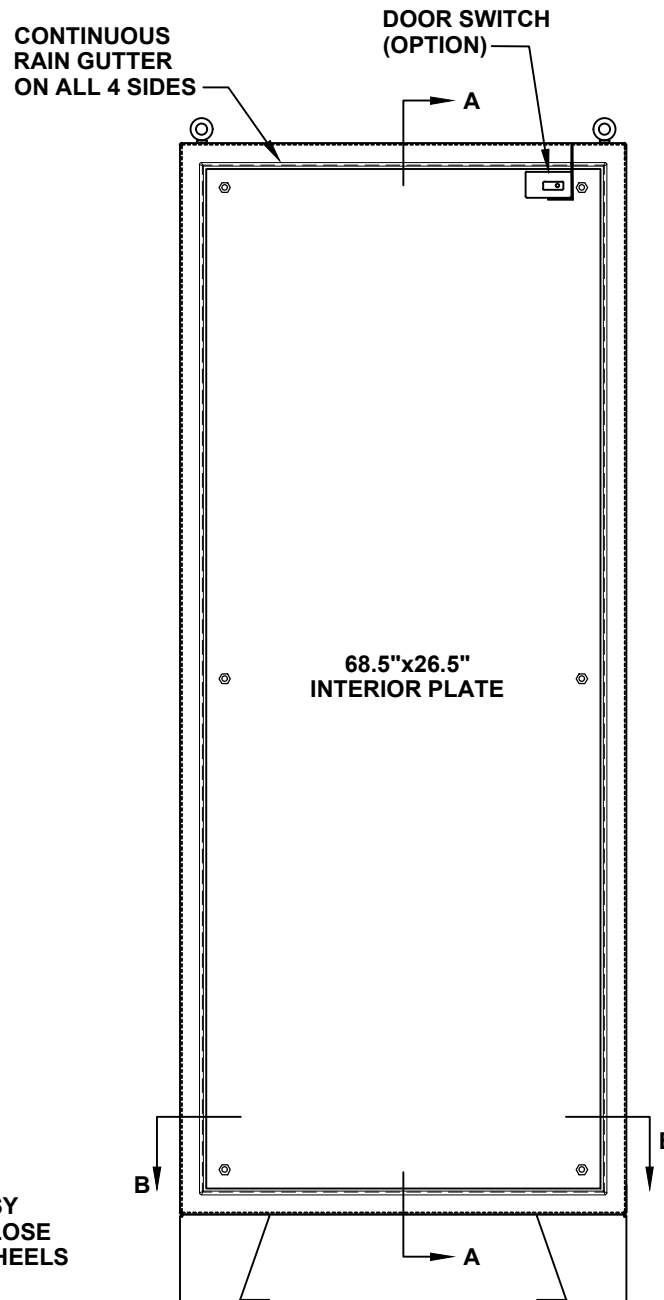
FRONT VIEW WITH DOOR REMOVED
