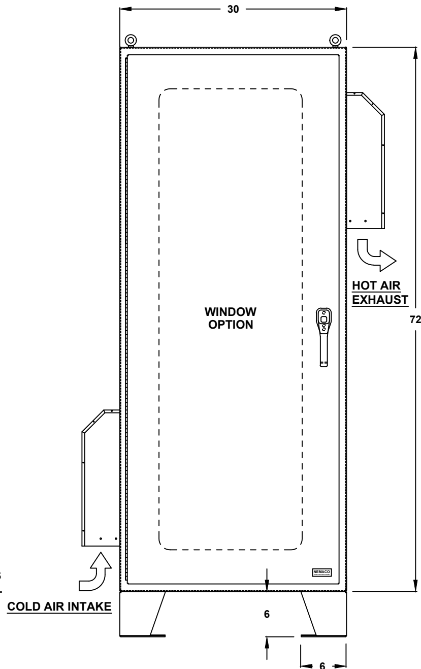
FRONT VIEW
