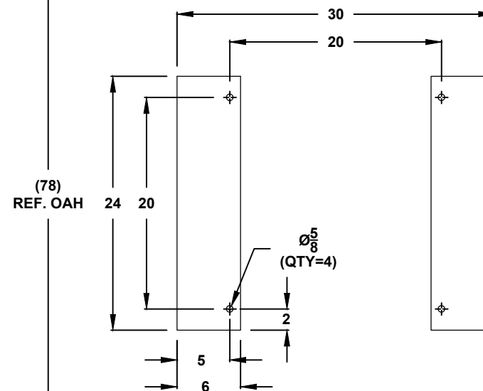
CROSS SECTION VIEW C-C MOUNTING HOLES
