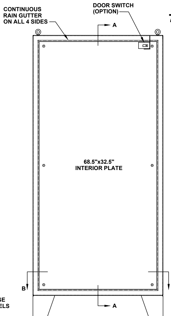
FRONT VIEW WITH DOOR REMOVED
