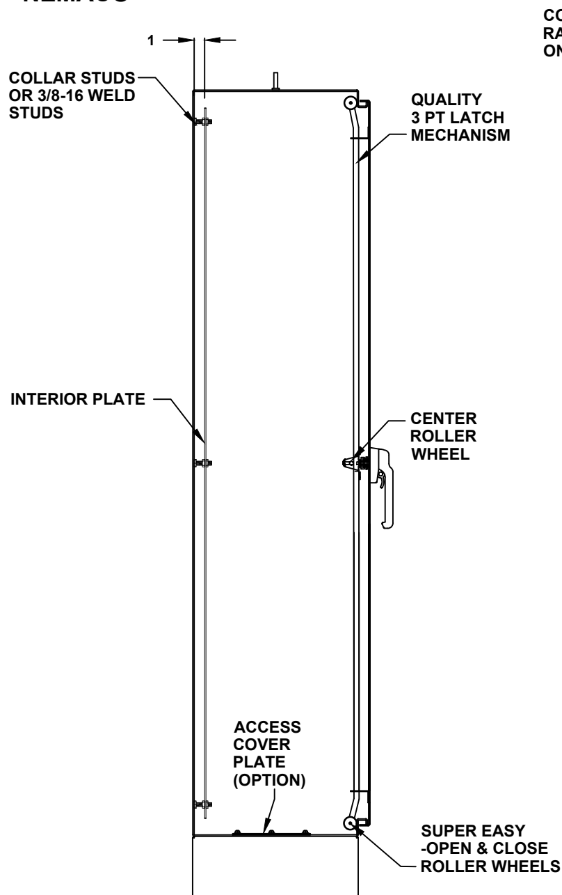
CROSS SECTION VIEW A-A
