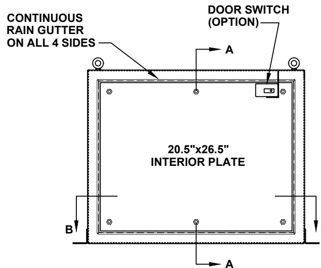
FRONT VIEW WITH DOOR REMOVED
