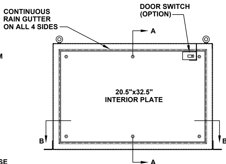
FRONT VIEW WITH DOOR REMOVED
