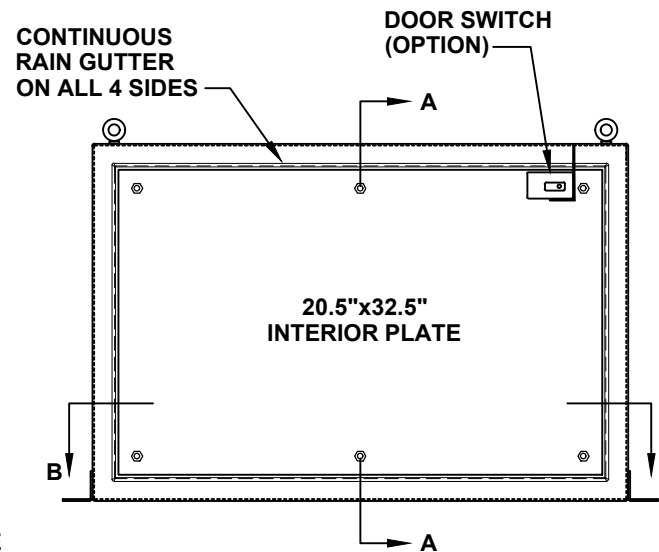
FRONT VIEW WITH DOOR REMOVED
