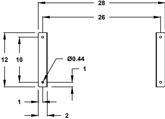
CROSS SECTION VIEW C-C MOUNTING HOLES
