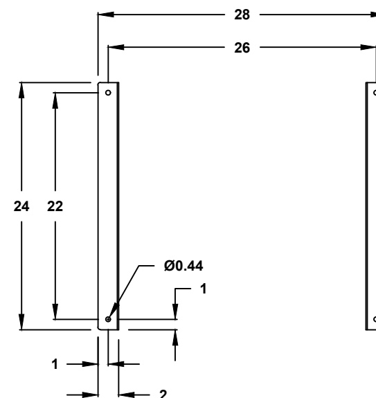
CROSS SECTION VIEW C-C MOUNTING HOLES
