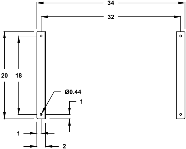
CROSS SECTION VIEW C-C MOUNTING HOLES
