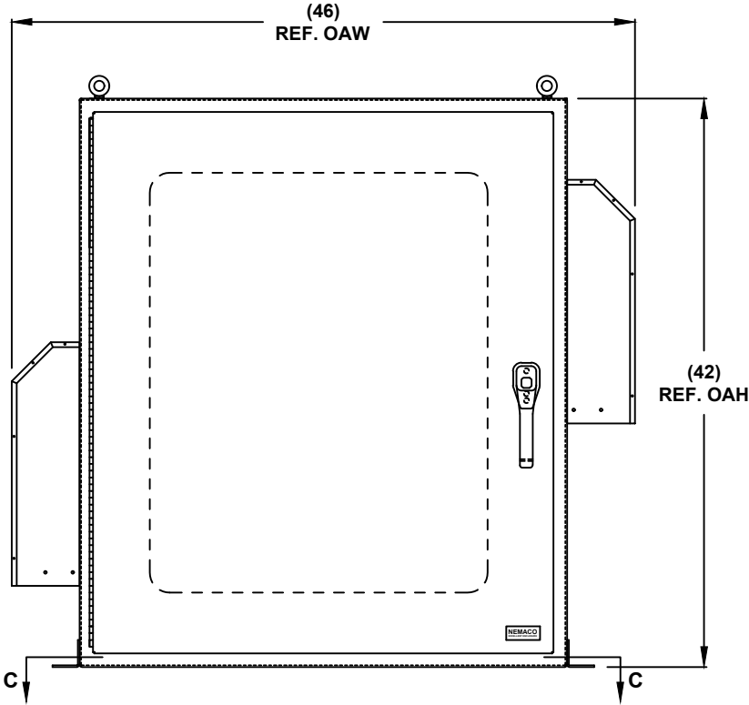
FRONT VIEW
