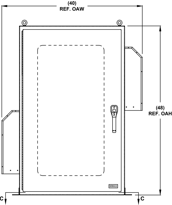
FRONT VIEW
