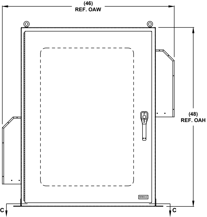
FRONT VIEW
