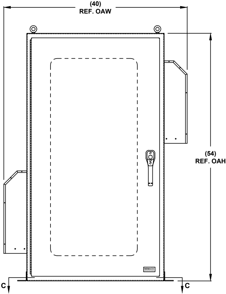
FRONT VIEW
