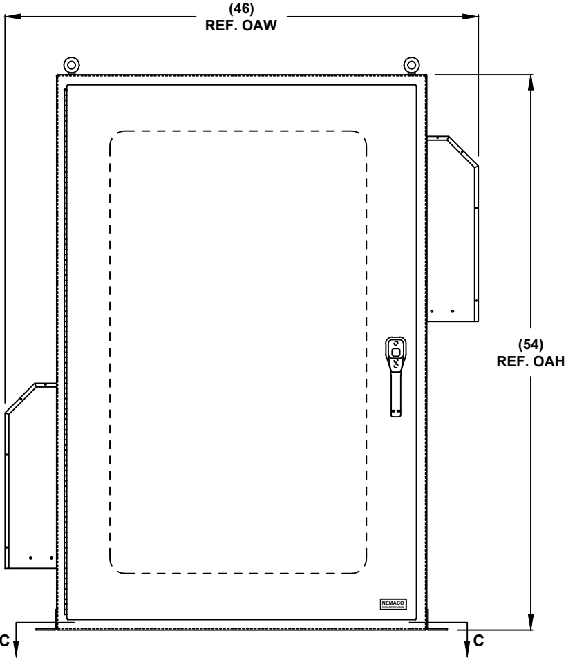
FRONT VIEW
