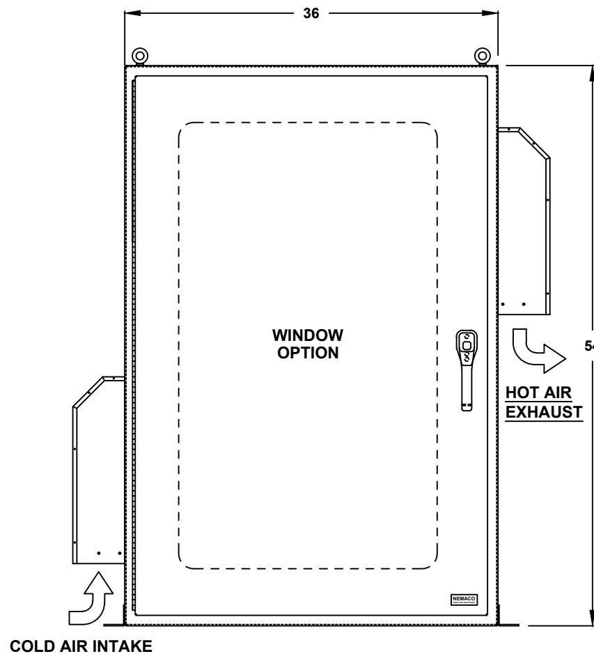
FRONT VIEW
