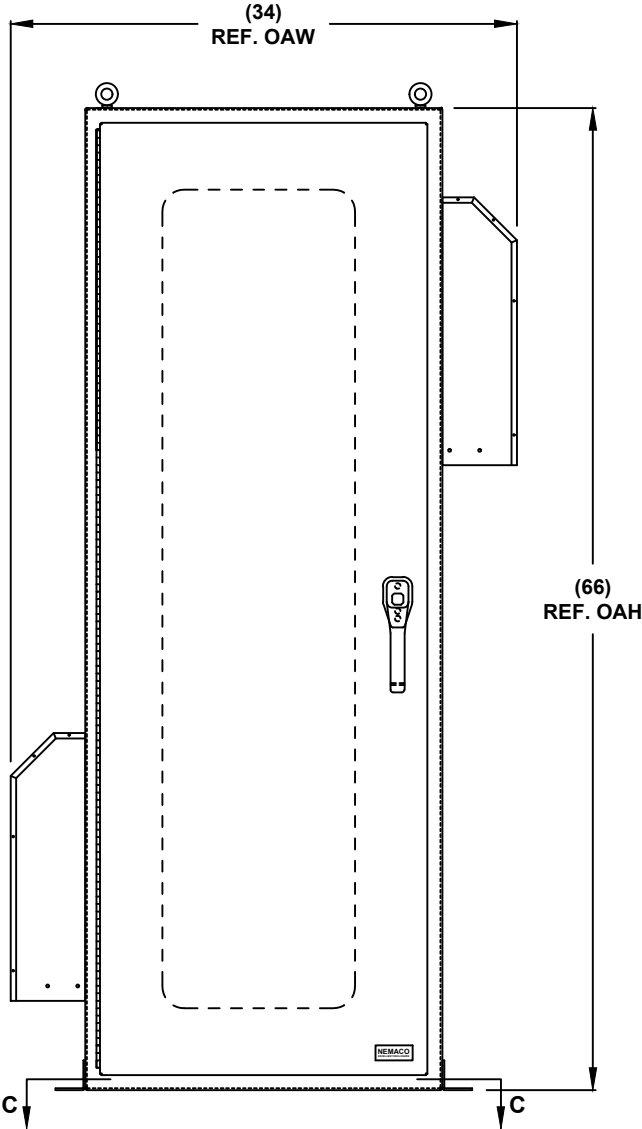
FRONT VIEW
