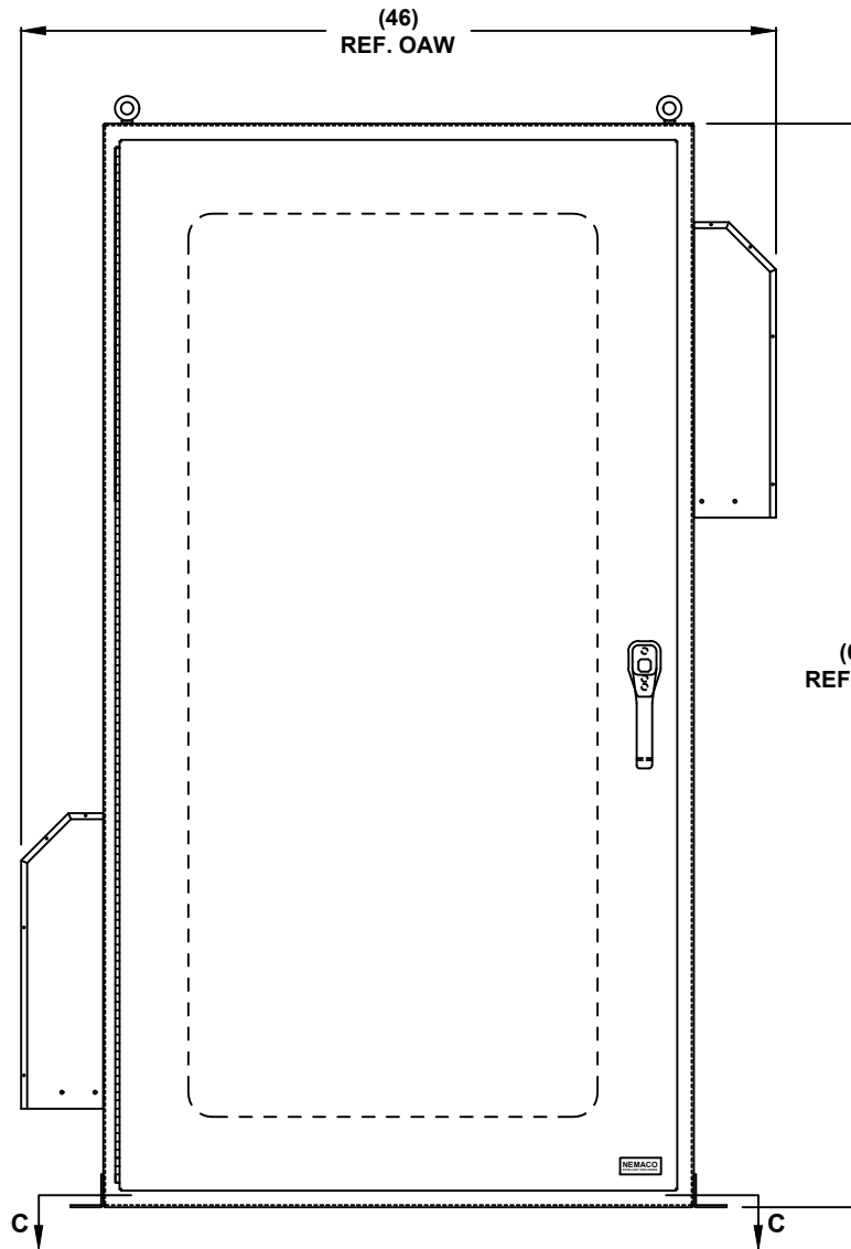
FRONT VIEW
