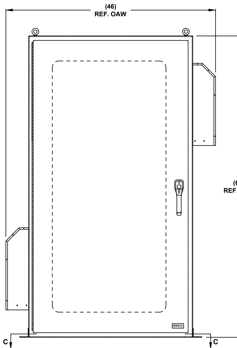
FRONT VIEW
