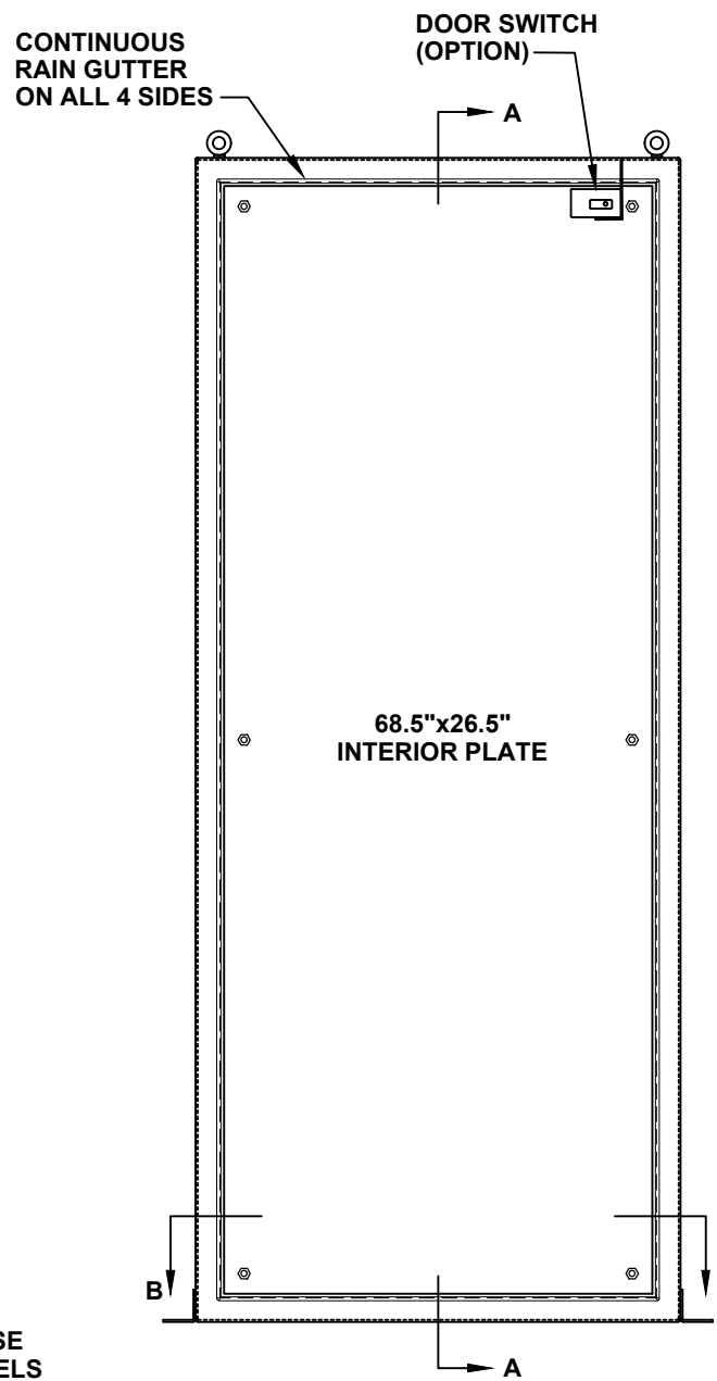
FRONT VIEW WITH DOOR REMOVED
