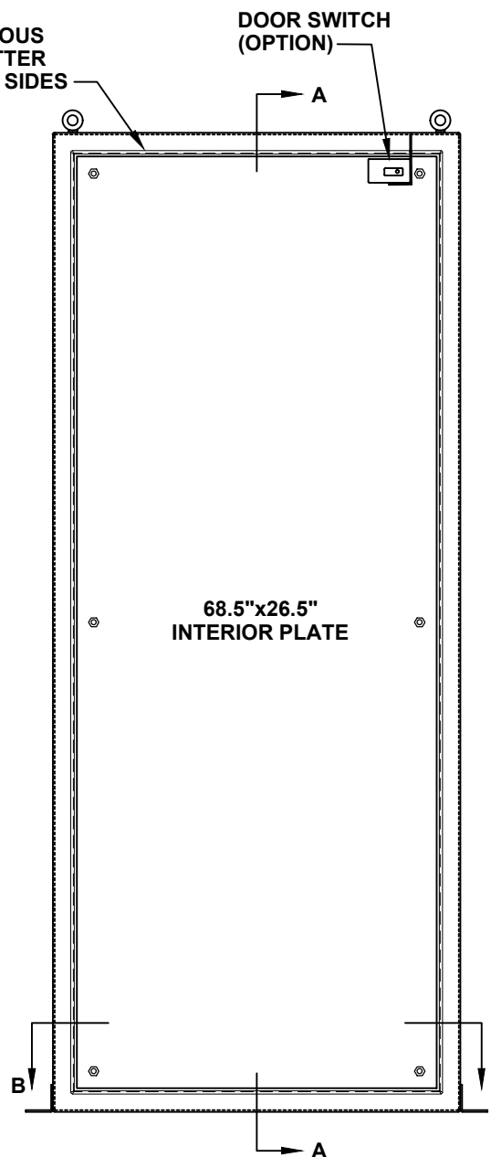
FRONT VIEW WITH DOOR REMOVED
