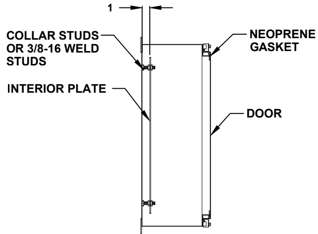
CROSS SECTION VIEW A-A
