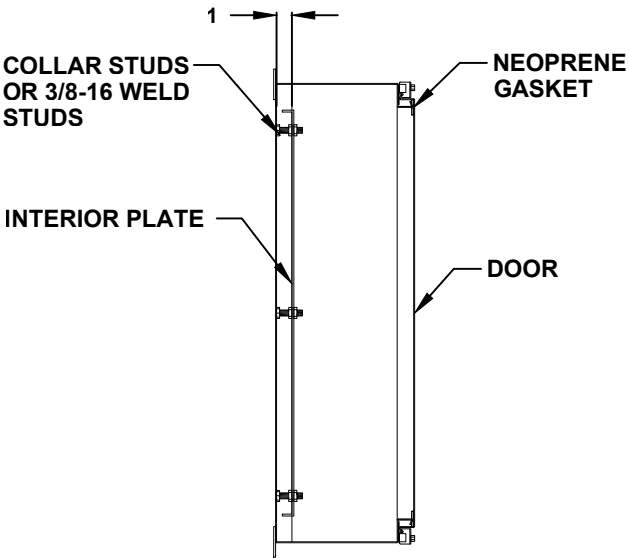
CROSS SECTION VIEW A-A
