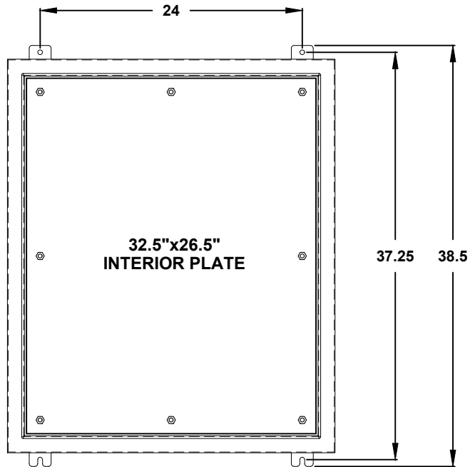
FRONT VIEW WITH DOOR REMOVED
