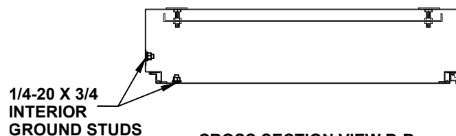
CROSS SECTION VIEW B-B
