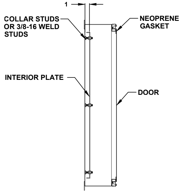
CROSS SECTION VIEW A-A
