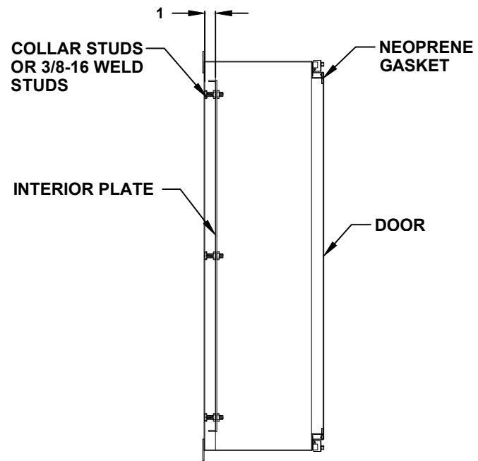
CROSS SECTION VIEW A-A
